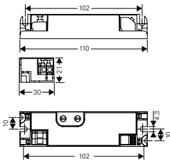
Module housing
