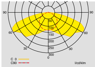
Polar curve SV EURO 1 with clear cover
